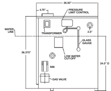
RIGHT SIDE
